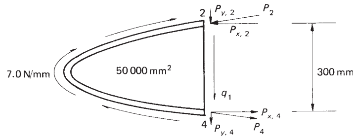
Fig. 24.10 Equilibrium of nose portion of the rib.
